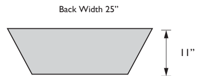
Back Width 25" Front Width 13" 20853, 20854, 20855 Plan View
